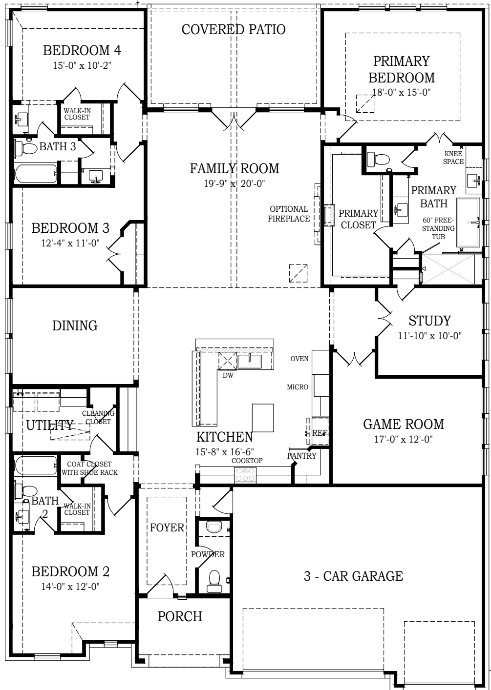
FLOOR PLAN
