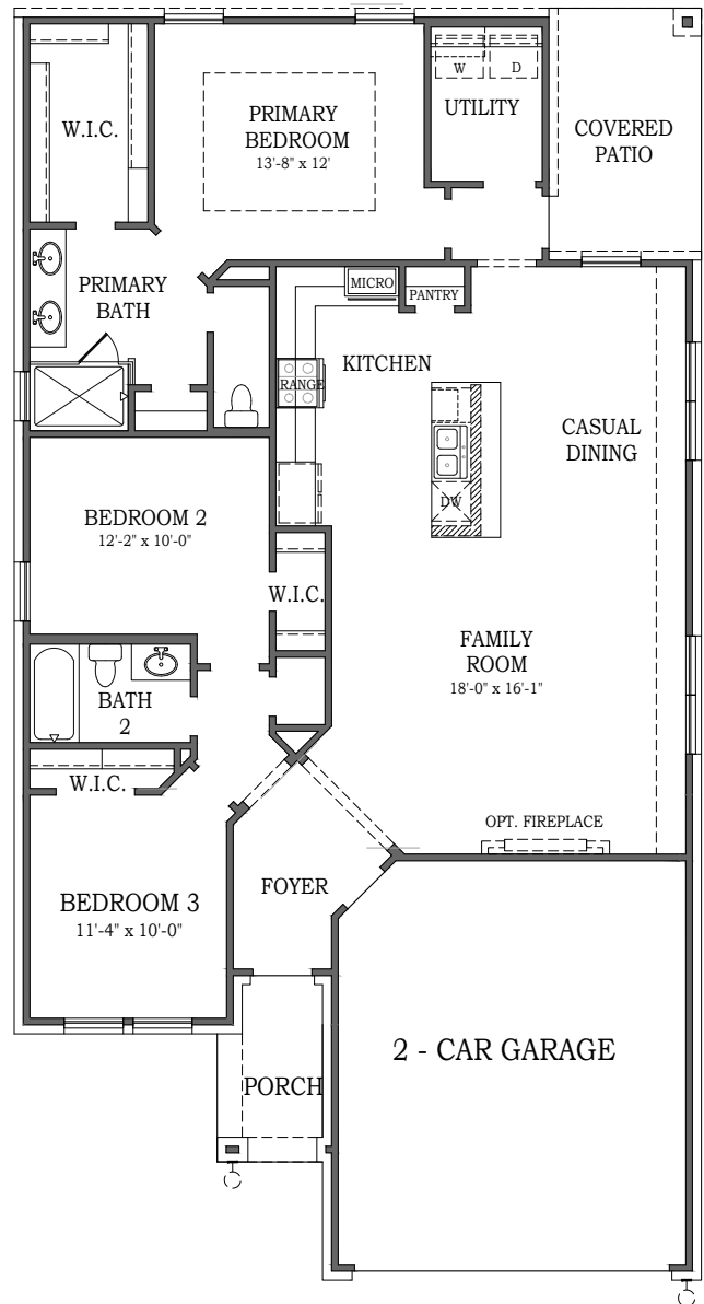
FLOOR PLAN
