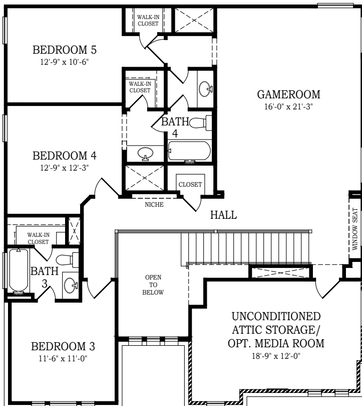
SECOND FLOOR
