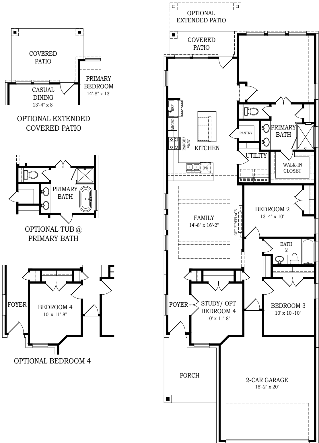
FLOOR PLAN - ELEVATION A2
