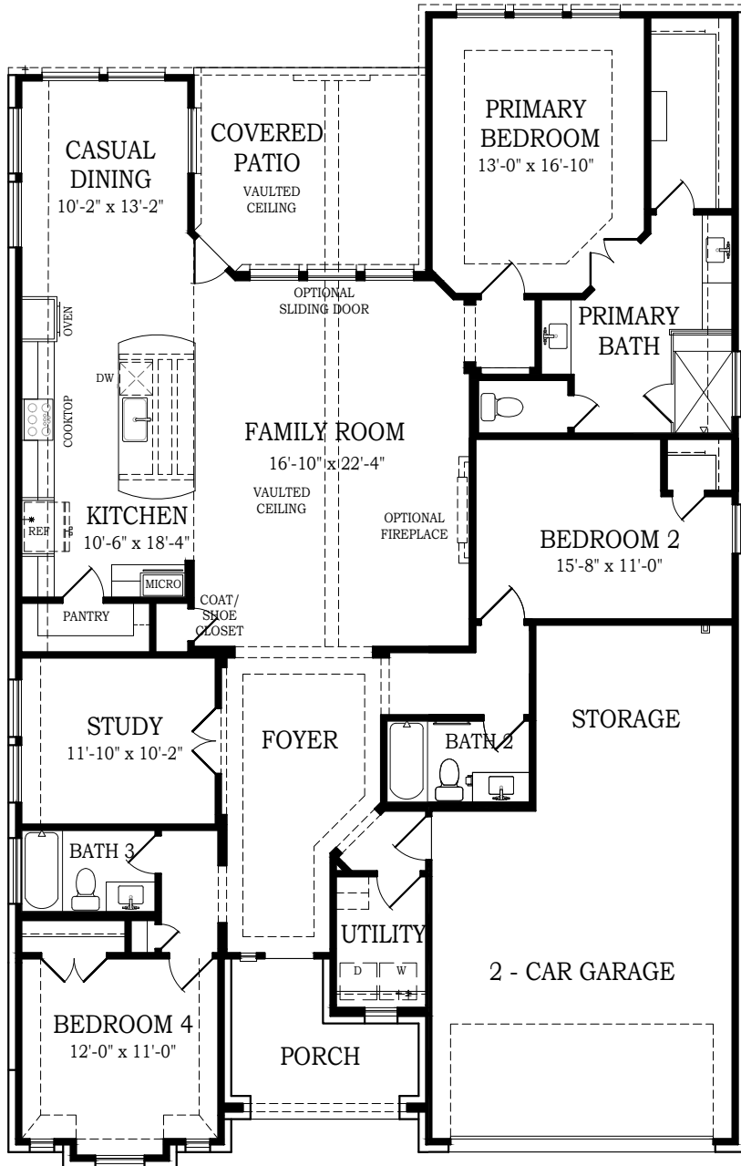
FLOOR PLAN
