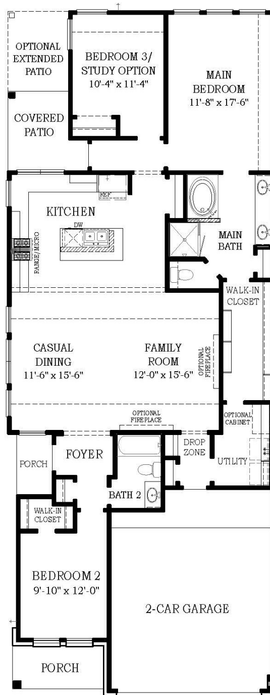
FLOOR PLAN
