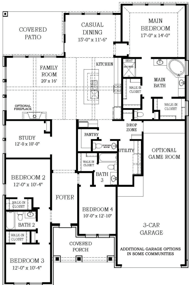
FLOOR PLAN
